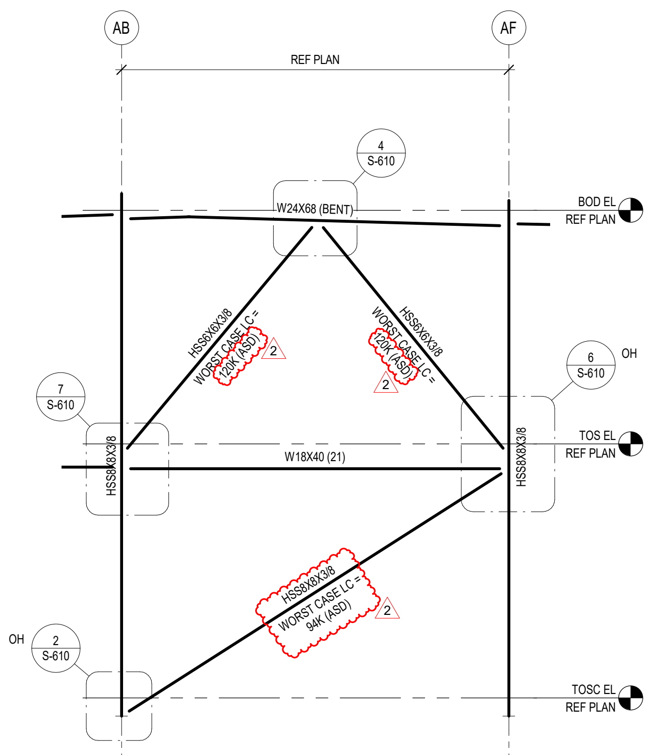
1 BRACE ELEVATION
