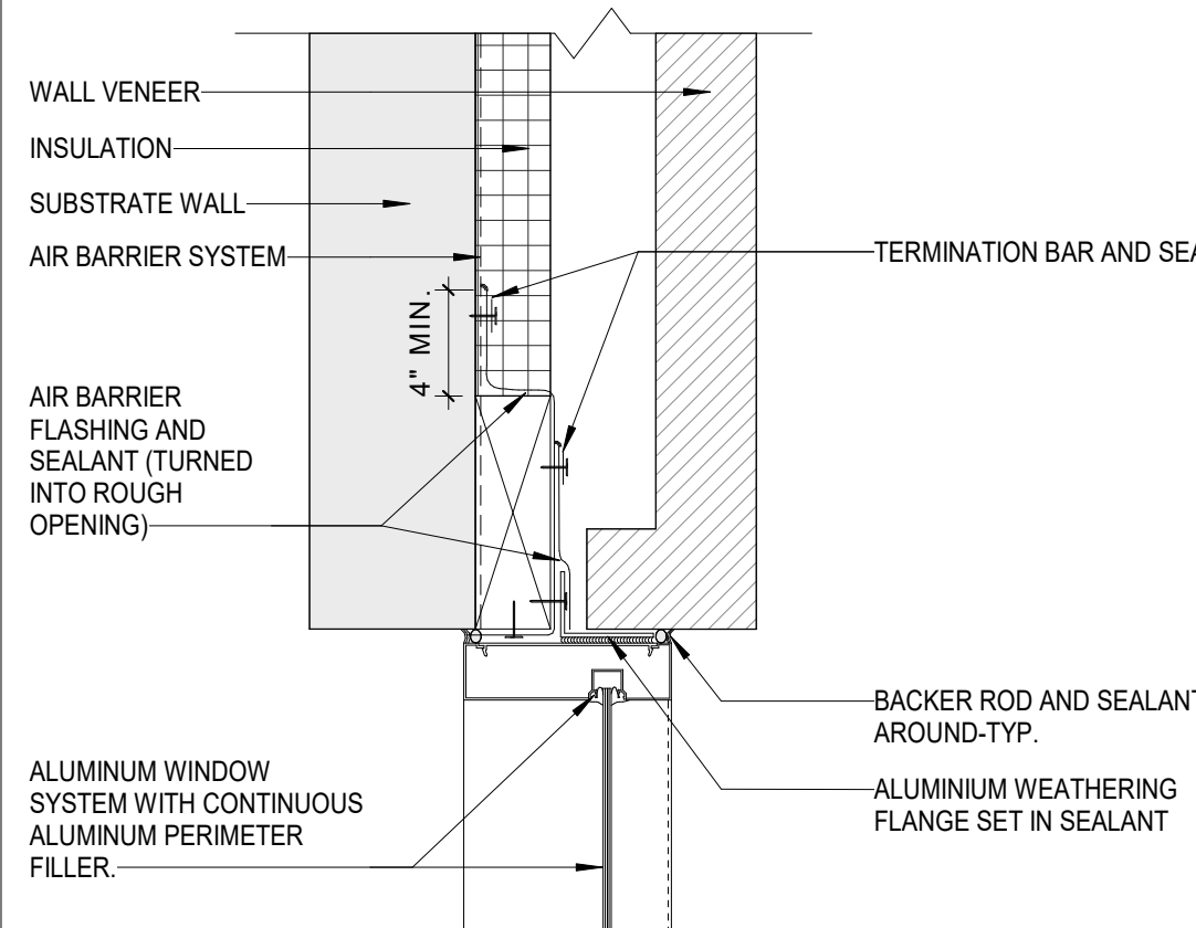
25 STOREFRONT HEAD AT LOOSE LINTEL NOT TO SCALE
