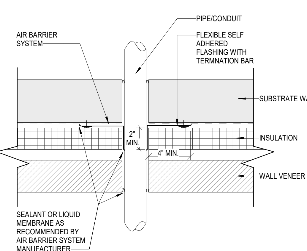
15 PIPE/CONDUIT WALL PENETRATION NOT TO SCALE
