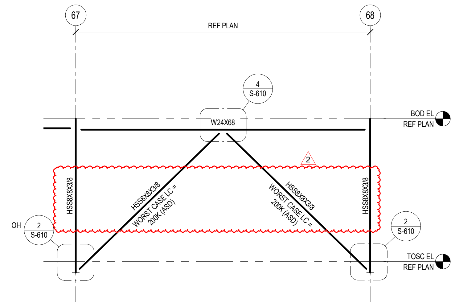
1 BRACE ELEVATION
