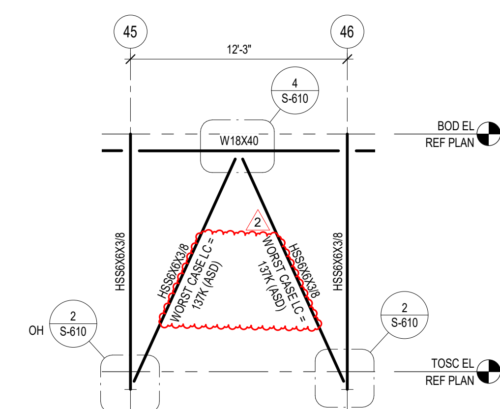
11 BRACE ELEVATION 3/16" = 1'-0"
