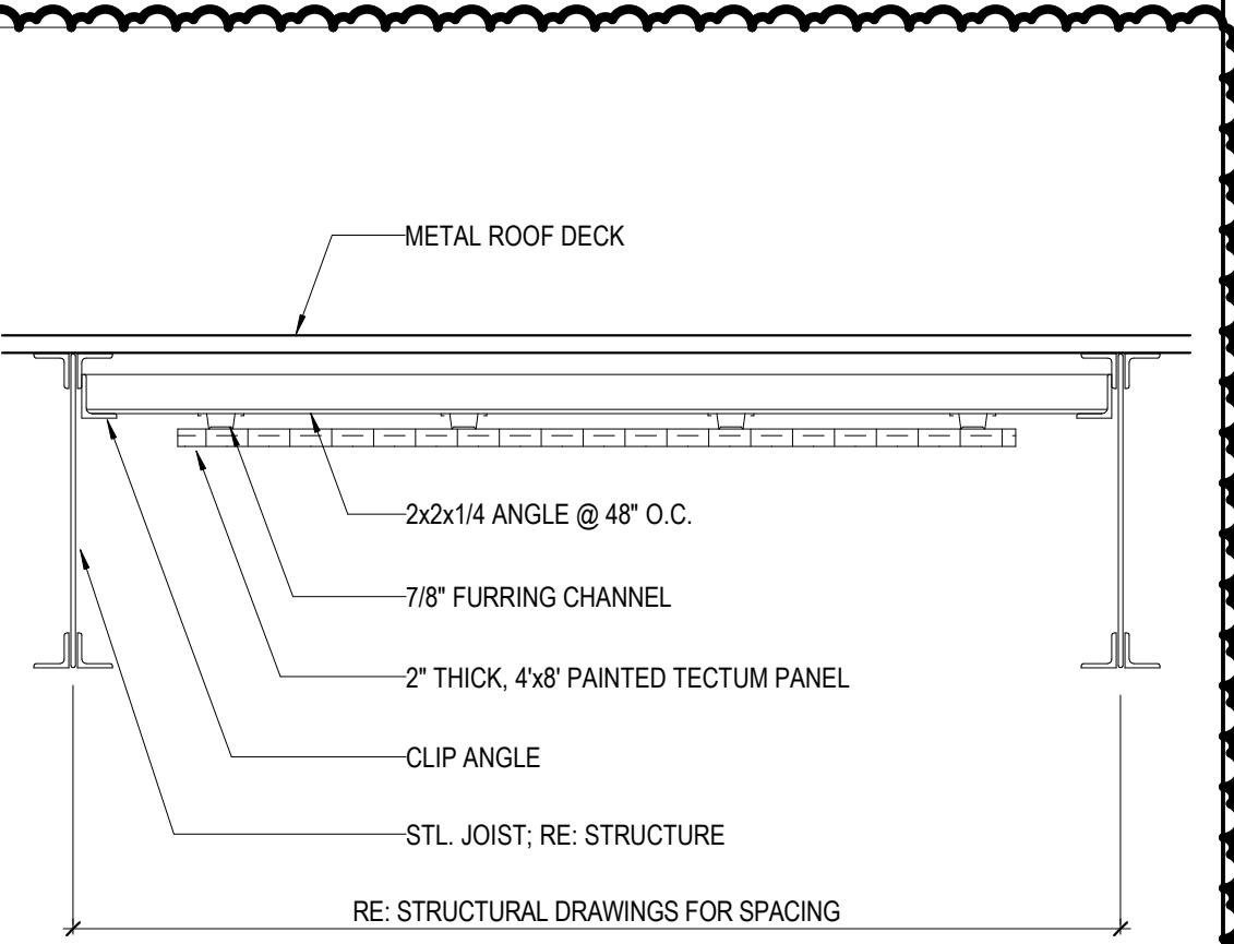
01 TECTUM PANEL DETAIL @ GYM 1" = 1'-0"
