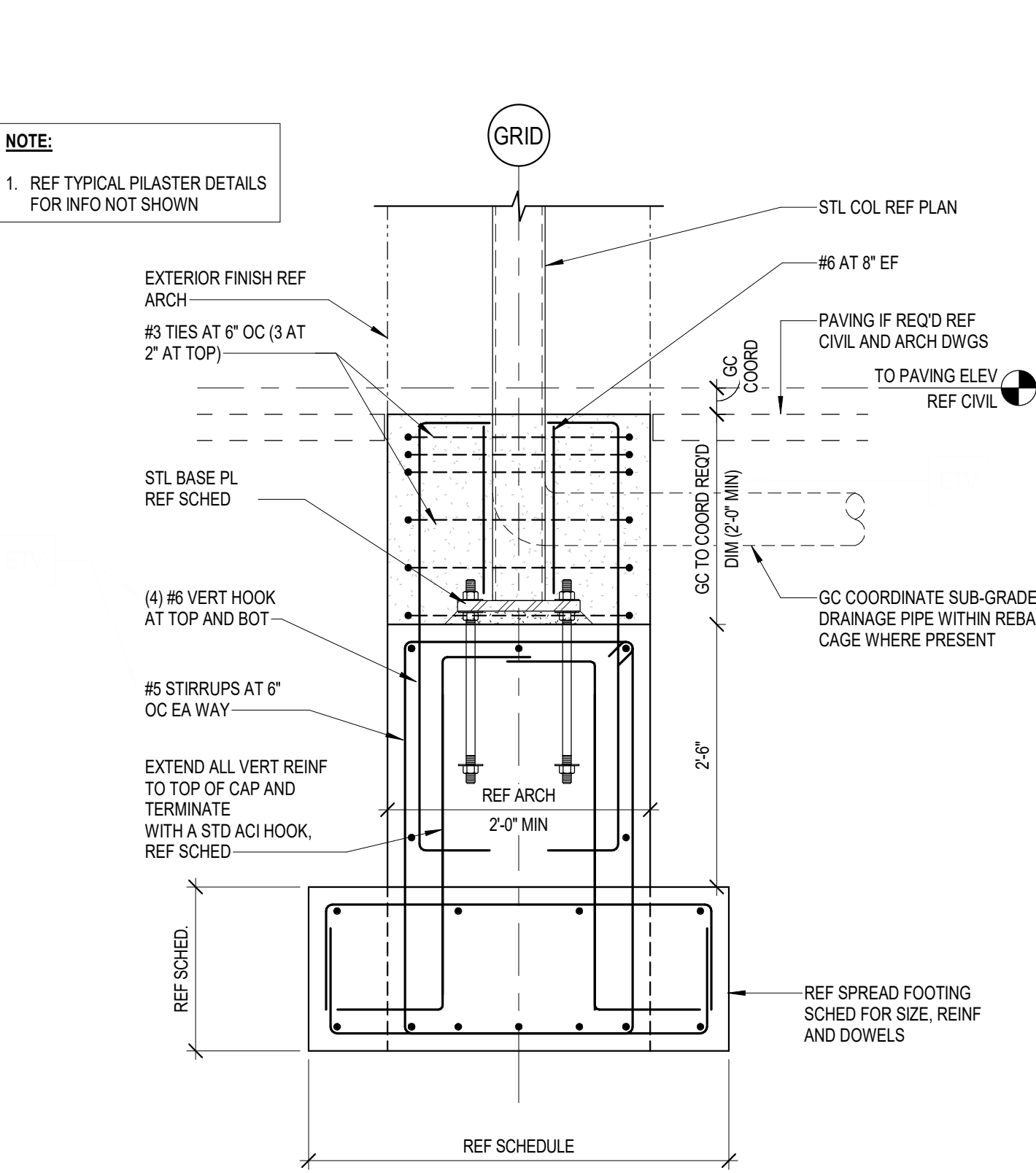
2 CANOPY COLUMN FOUNDATION 3/4" = 1'-0"
