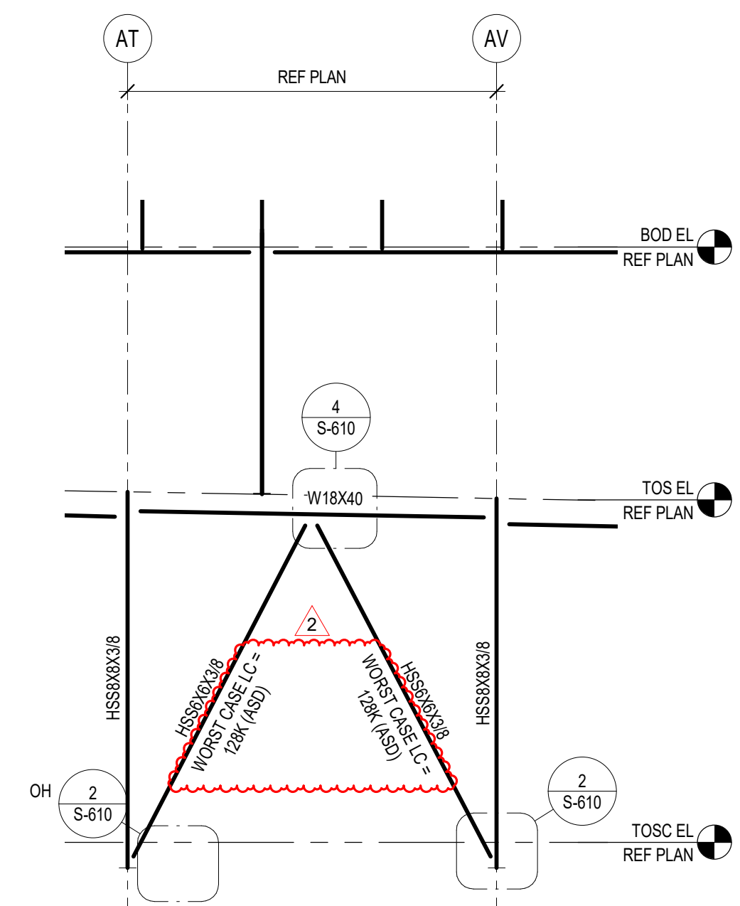
7 BRACE ELEVATION
