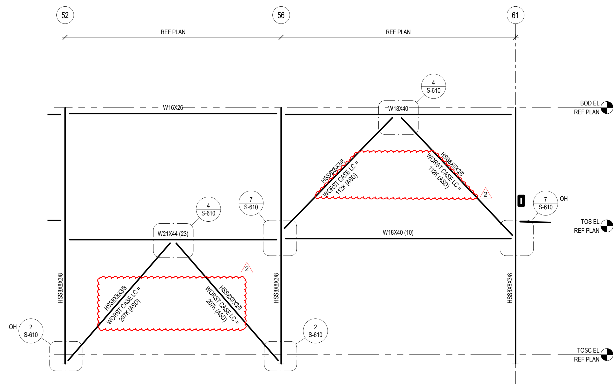
6 BRACE ELEVATION
