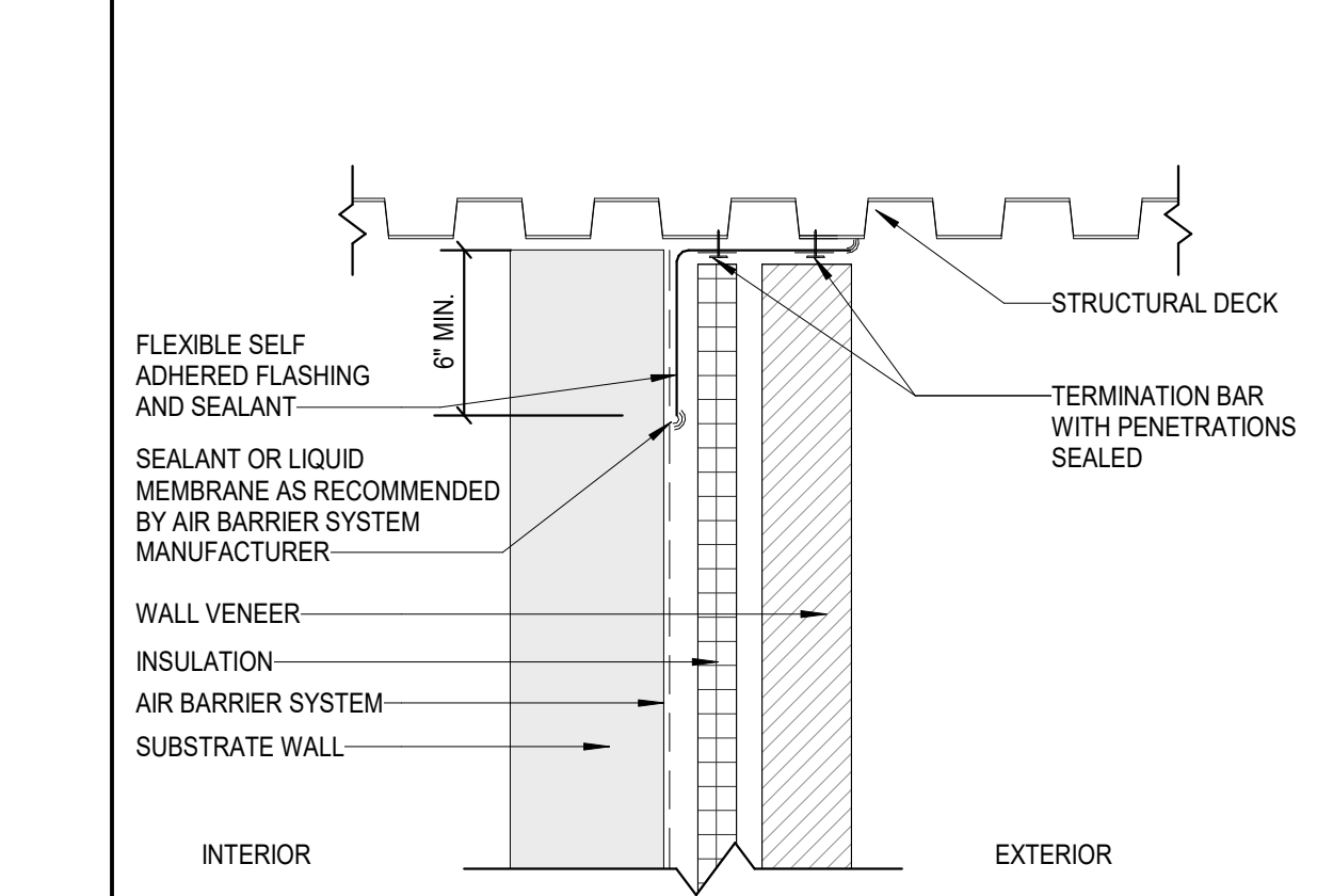
30 TOP OF WALL AT ROOF EDGE NOT TO SCALE
