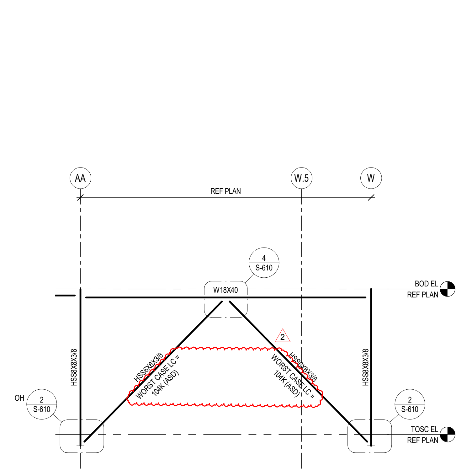
4 BRACE ELEVATION
