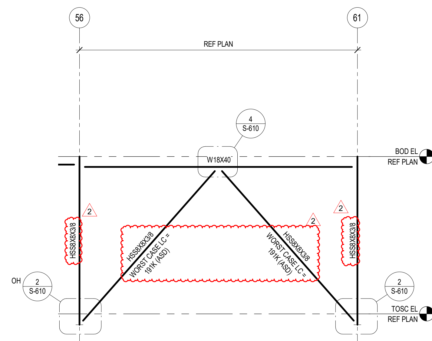
8 BRACE ELEVATION 3/16" = 1'-0"
