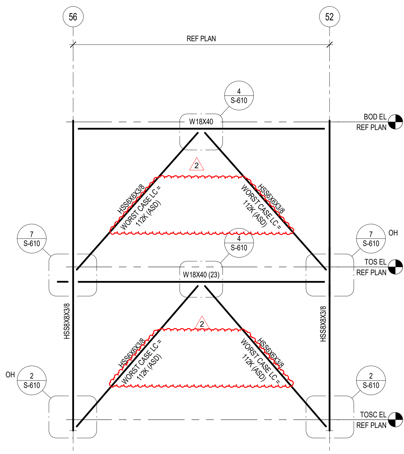
2 BRACE ELEVATION
