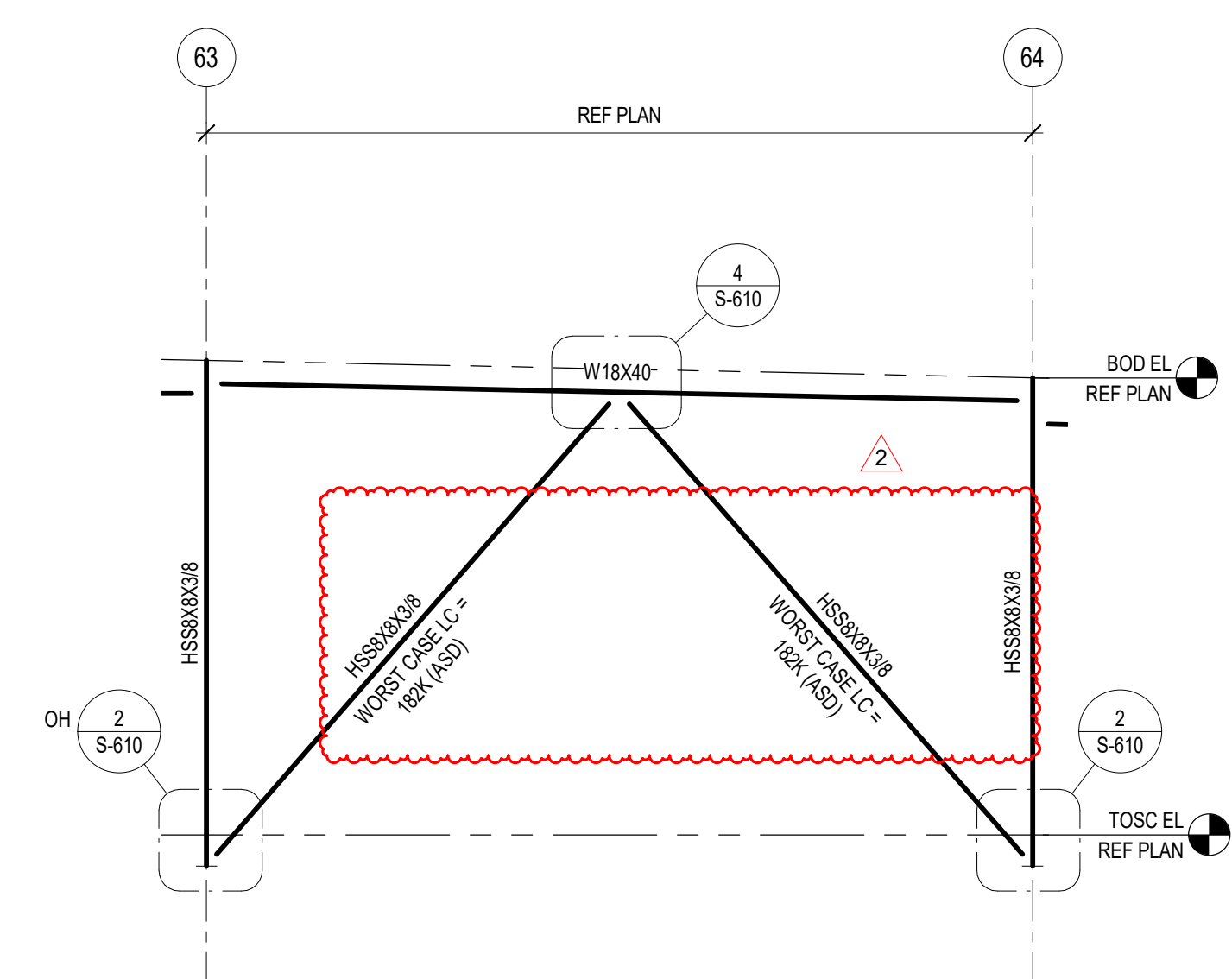
10 BRACE ELEVATION
