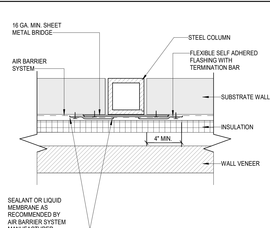
29 STEEL COLUMN CONNECTION NOT TO SCALE
