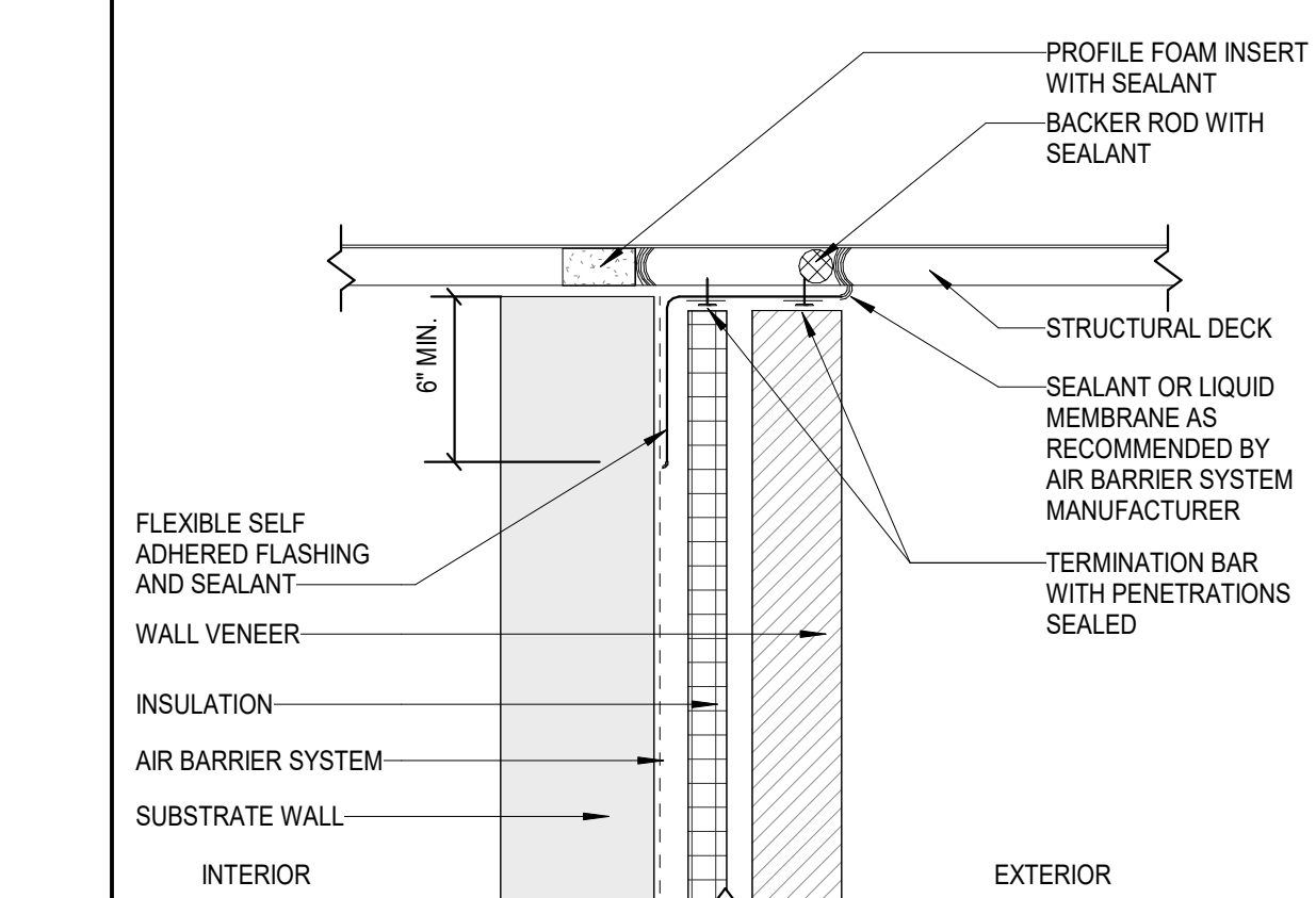
24 TOP OF WALL AT MTL. DECK NOT TO SCALE
