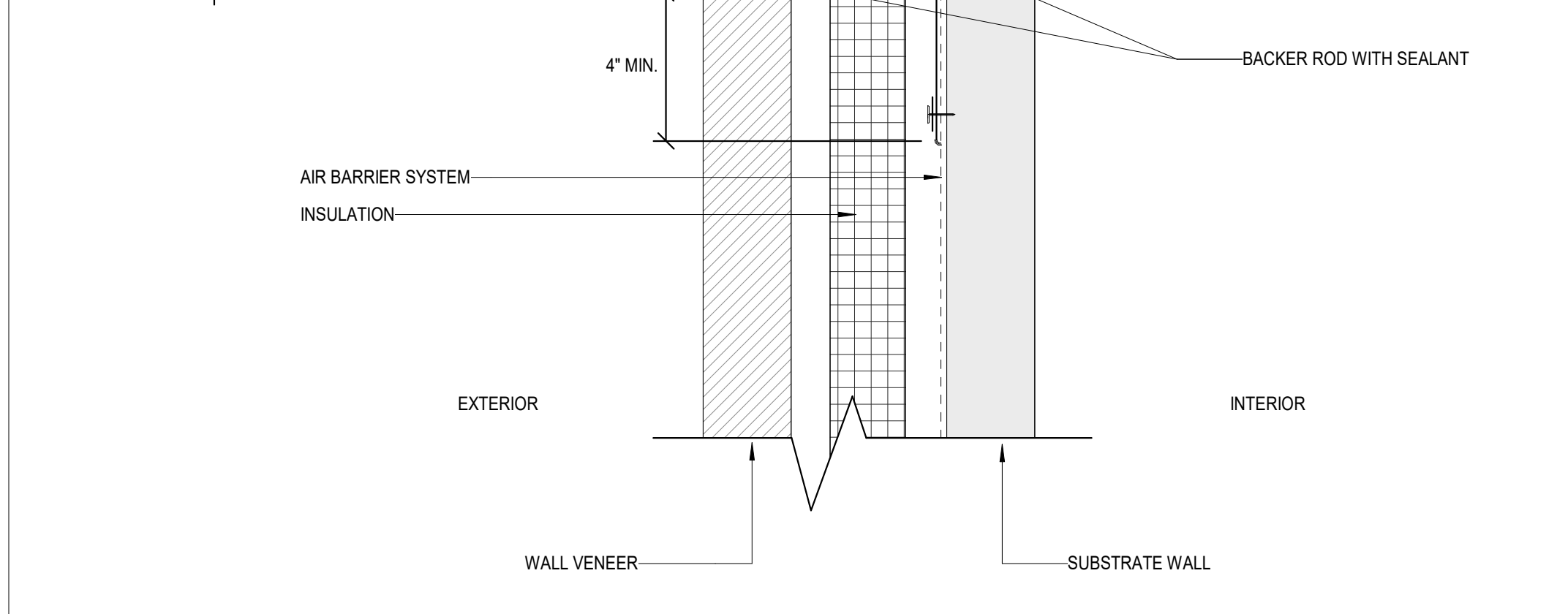
22 "T" CONNECTION EXPANSION JOINT NOT TO SCALE
