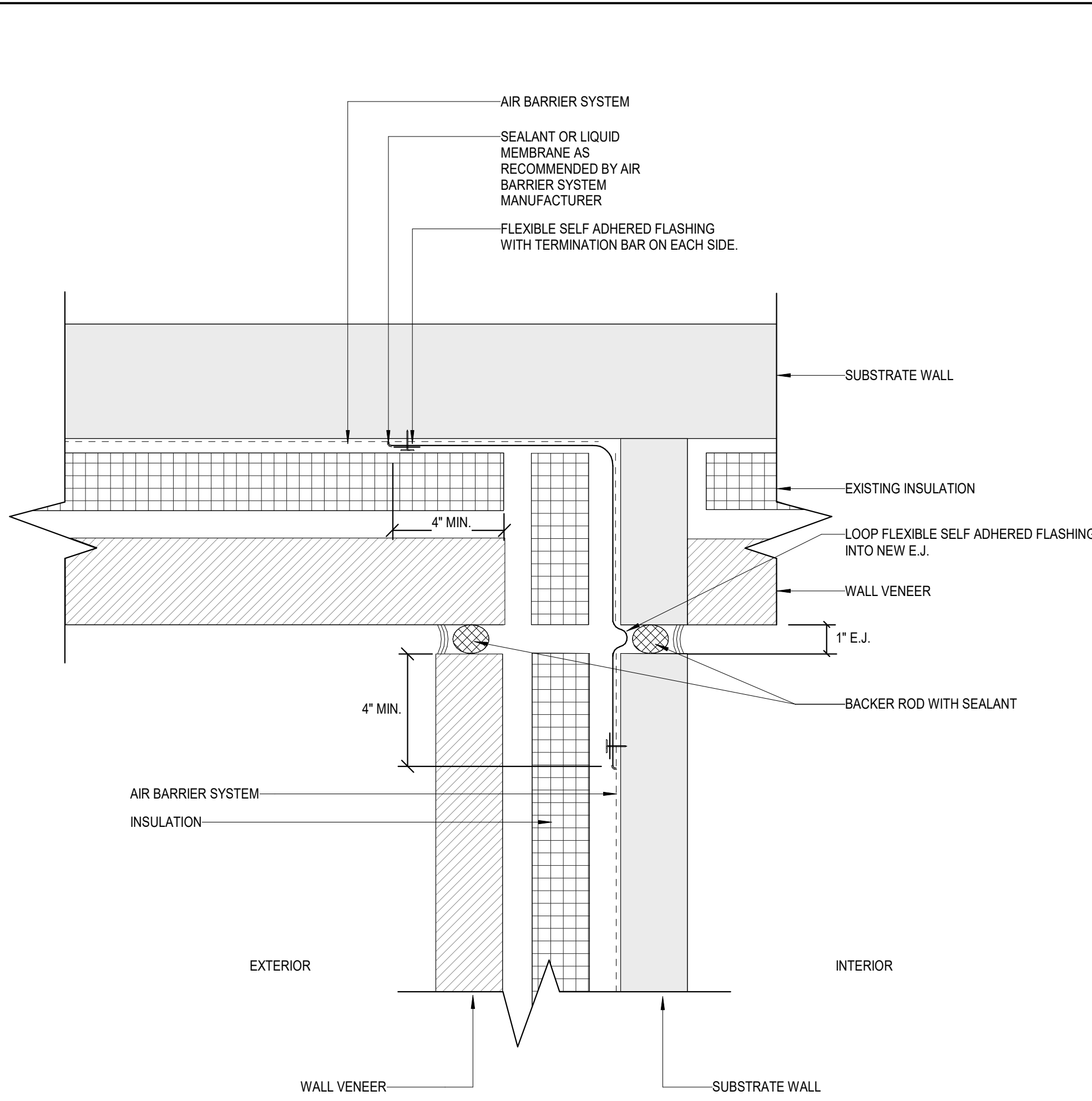
22 "T" CONNECTION EXPANSION JOINT NOT TO SCALE
