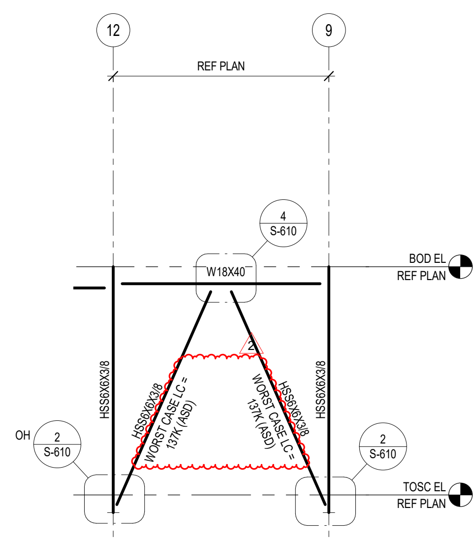
6 BRACE ELEVATION
