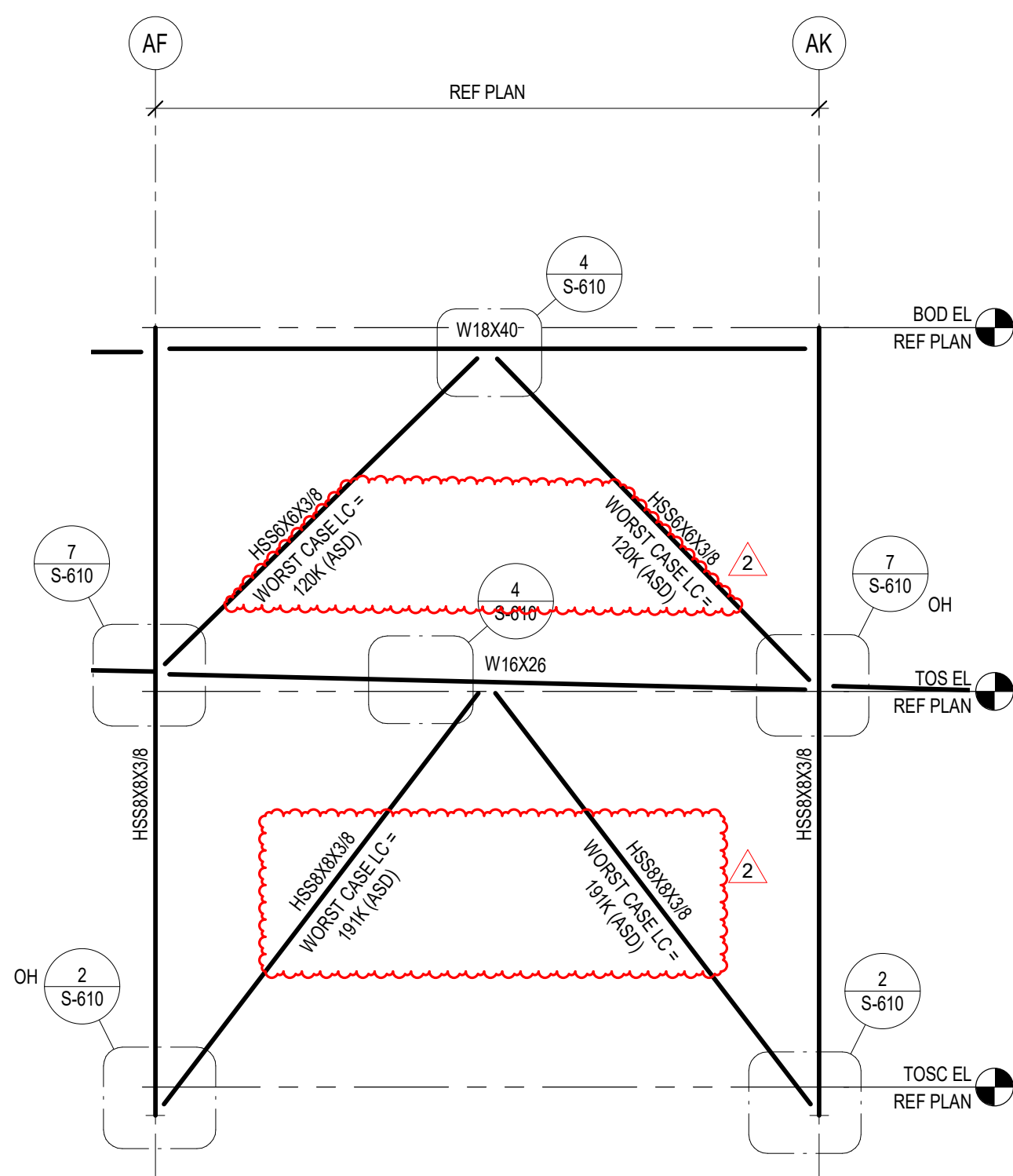
3 BRACE ELEVATION
