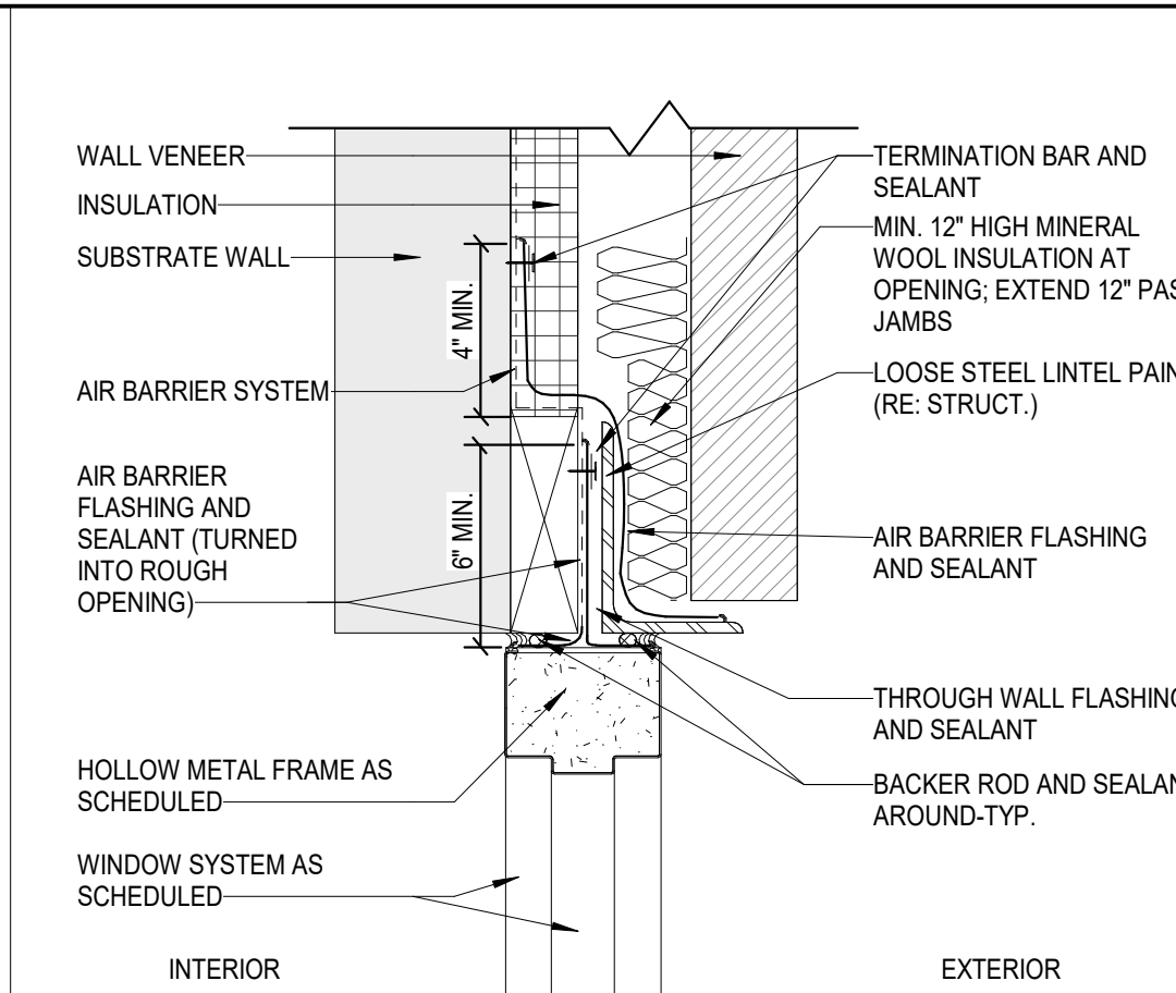
26 HOLLOW METAL HEAD NOT TO SCALE
