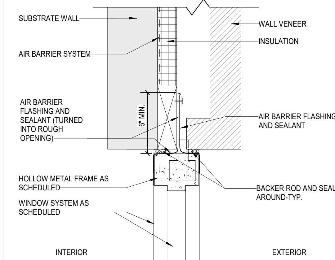
26 HOLLOW METAL HEAD NOT TO SCALE
