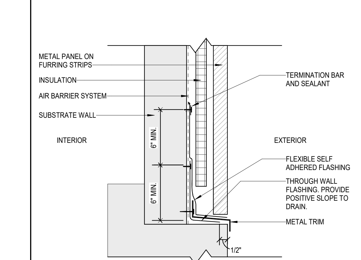
12 BASE OF METAL WALL PANEL NOT TO SCALE
