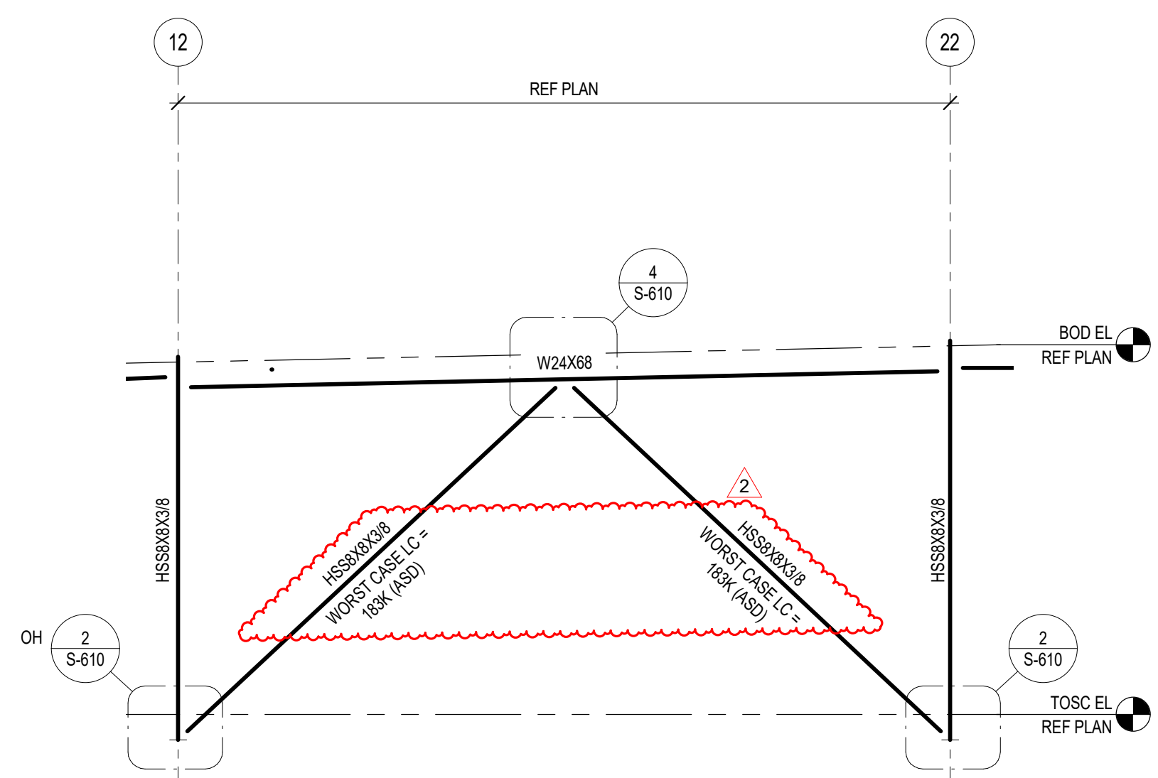
5 BRACE ELEVATION
