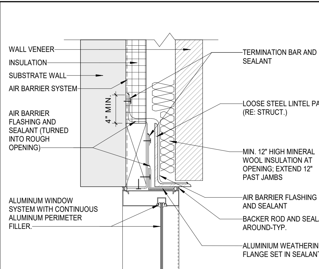
25 STOREFRONT HEAD AT LOOSE LINTEL NOT TO SCALE
