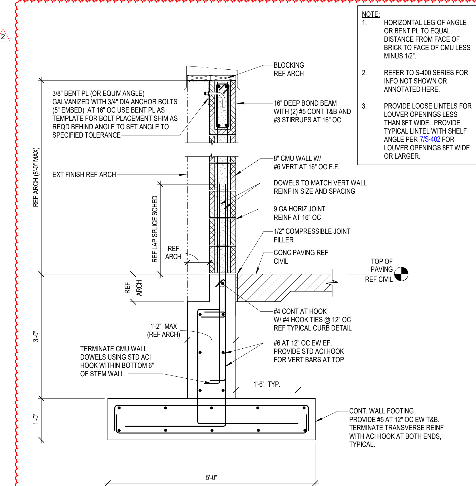
1 SCREEN WALL AT MECH YARD 3/4" = 1'-0"
