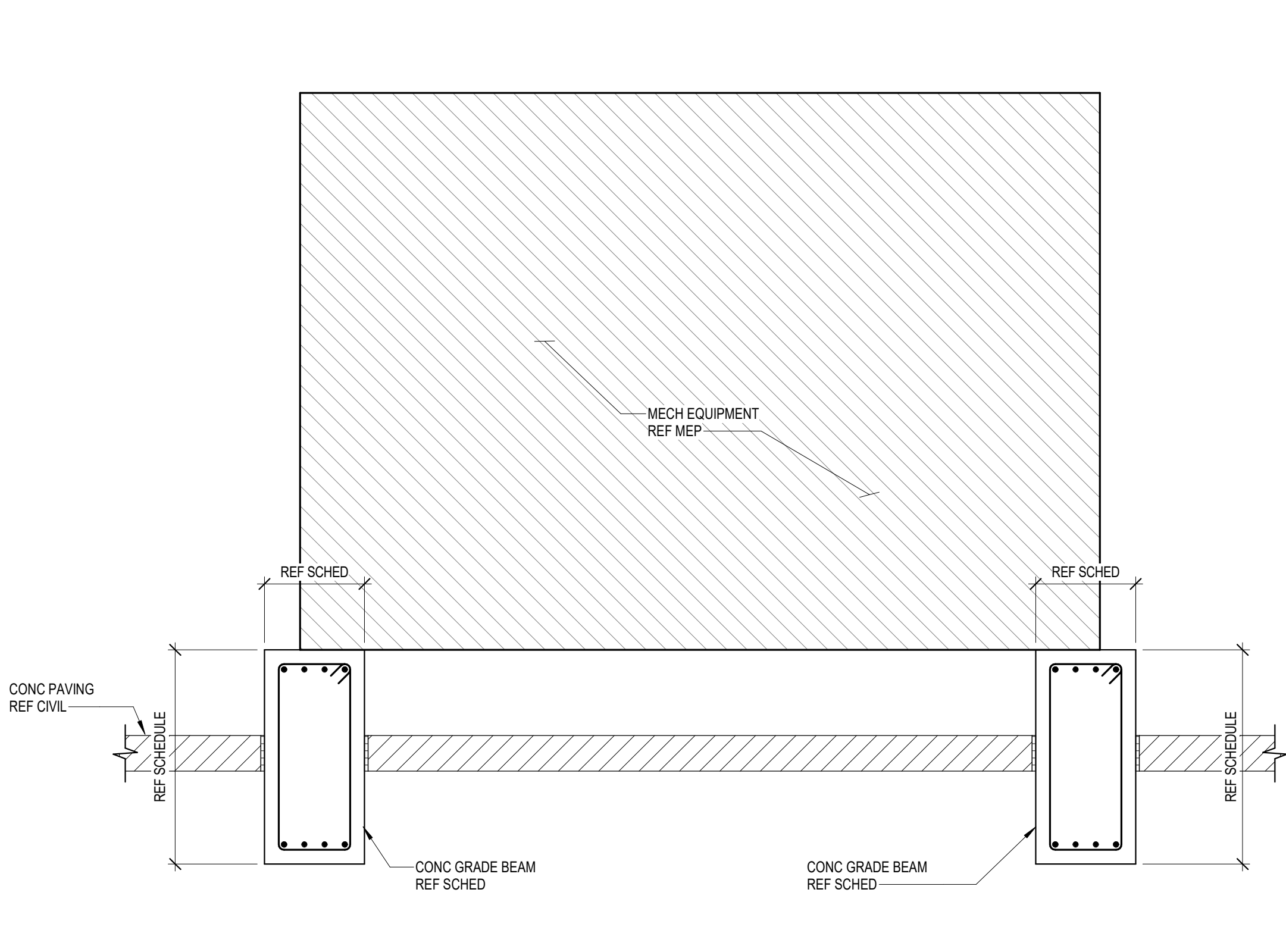
3 MECH EQUIPMENT SUPPORT 3/4" = 1'-0"
