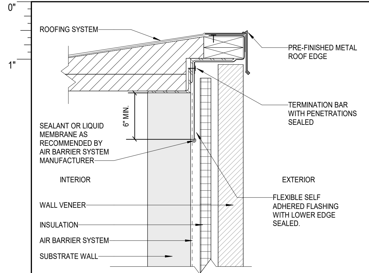
30 TOP OF WALL AT ROOF EDGE NOT TO SCALE
